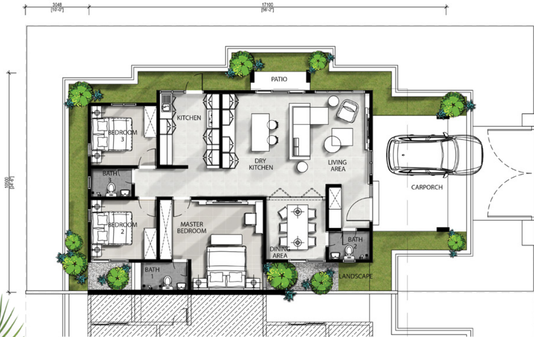
100 MASTER LAYOUT PLAN A3-1:75 SEMI-D 1 STOREY
